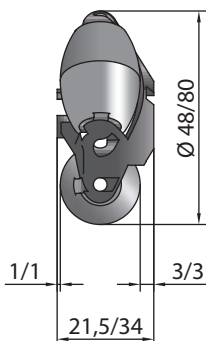
OmniWheel
