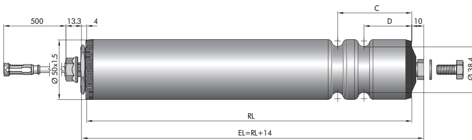
Fig.: With female thread
